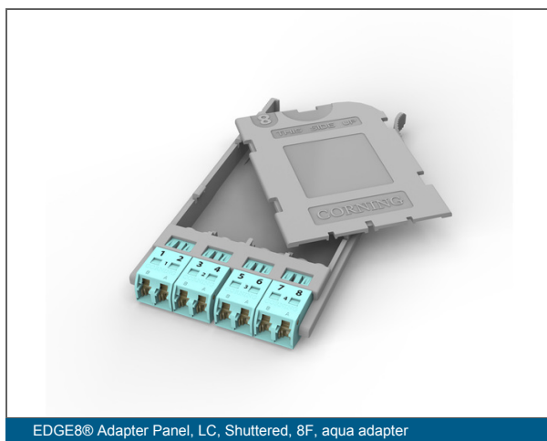
EDGE8® Adapter Panel, LC, Shuttered, 8F, aqua adapter
